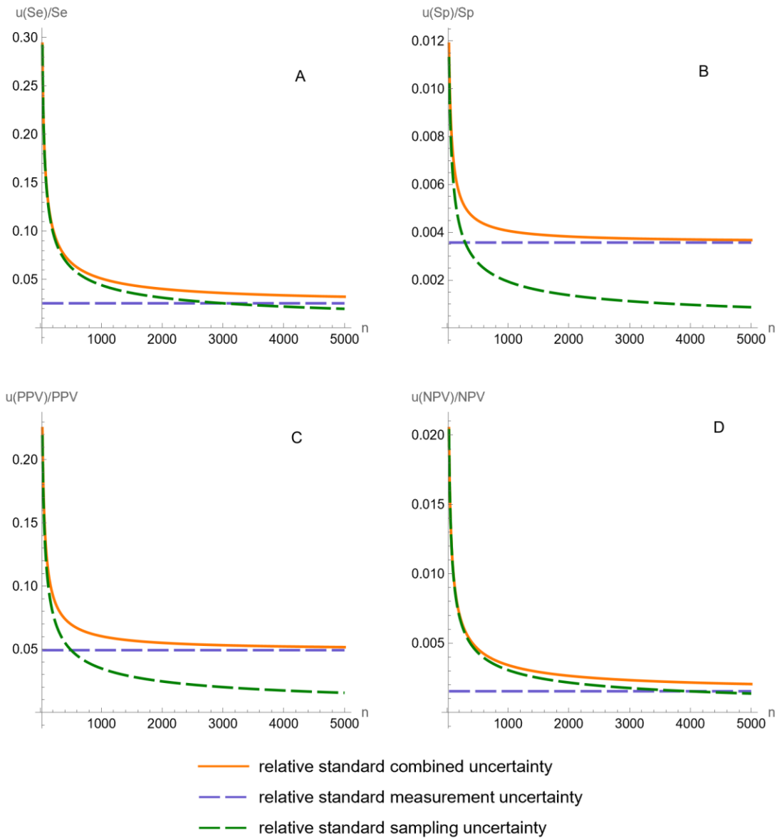
Figure 20. DAM standard uncertainties versus population sample size plots. Plots of relative standard combined, sampling, and measurement uncertainties of (A) sensitivity ( Se ), (B) specificity ( Sp ), (C) positive predictive value ( PPV ), and (D) negative predictive value ( NPV ) versus total population sample size ( n ) curves, with the respective parameters in Table 4.
