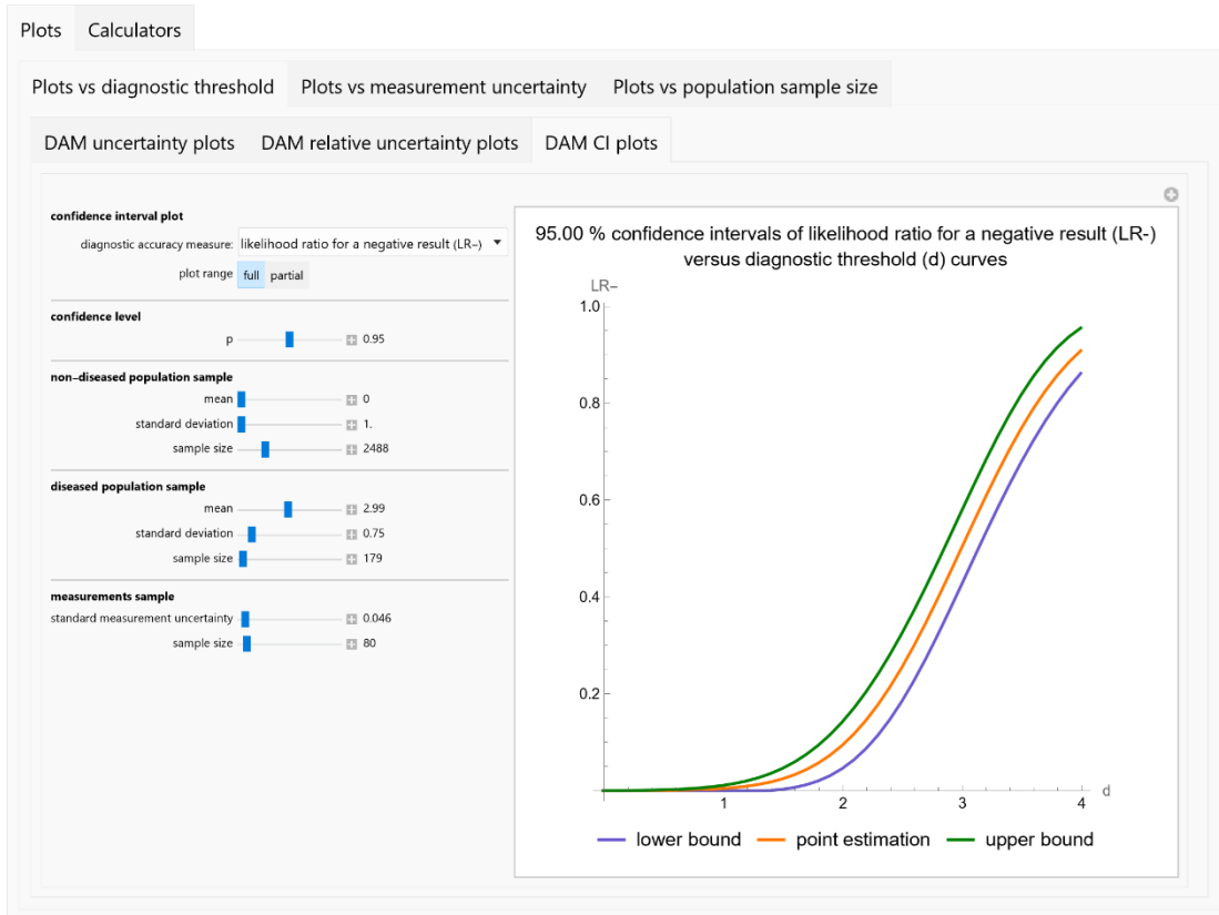
Figure 5. Plots vs diagnostic threshold module, DAM CI submodule screenshot. Confidence intervals of the likelihood ratio for a negative test result ( u(LR^-) ) versus diagnostic threshold ( d ) curves plot, with the settings shown at the left.
