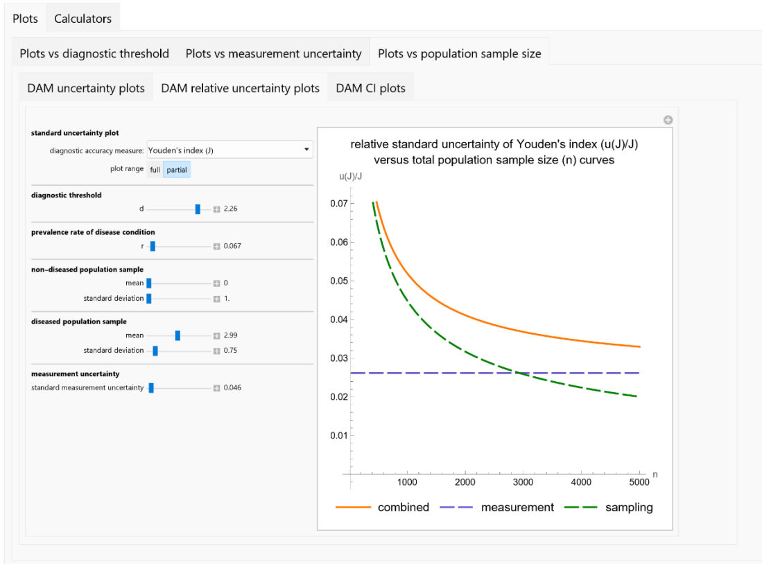
Figure 10. Plots vs. population sample size module, DAM relative uncertainty submodule screenshot. The relative standard combined, sampling, and measurement uncertainty of Youden's index ( u(J)/J ) versus total population sample size ( n ) curves plot, with the settings shown at the left.
