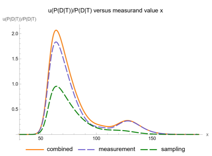
Figure 6. Relative standard sampling, measurement, and combined uncertainty of the posterior probability for diabetes versus FPG curve plot, with the settings of the program in Table 2.
