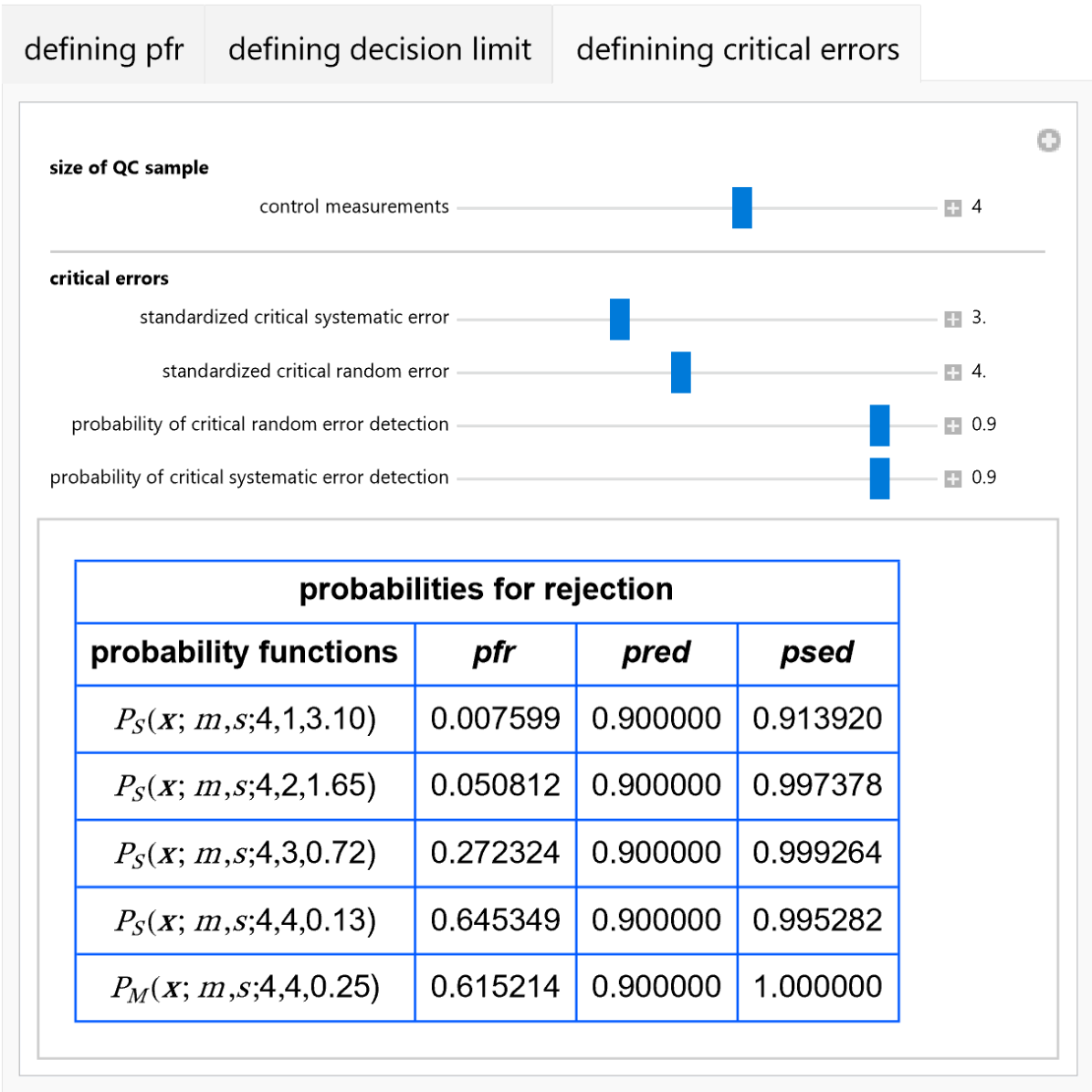
Figure 4: The probabilities for false rejection and critical error detection of the QC rules shown at the left of the table, with the settings shown at the top.
