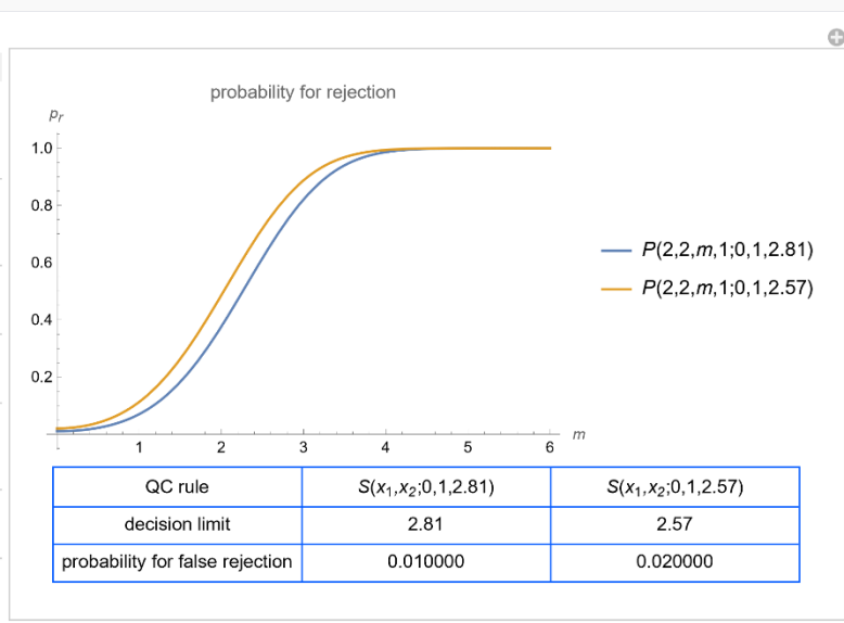
Figure 3: The probabilities for rejection of two alternative QC rules vs the standardized observed mean m of the control measurements, with the settings shown at the left.
